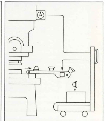
④カム入力・コンベア連動 Cam switch-belt conveyer interlocking operation.
